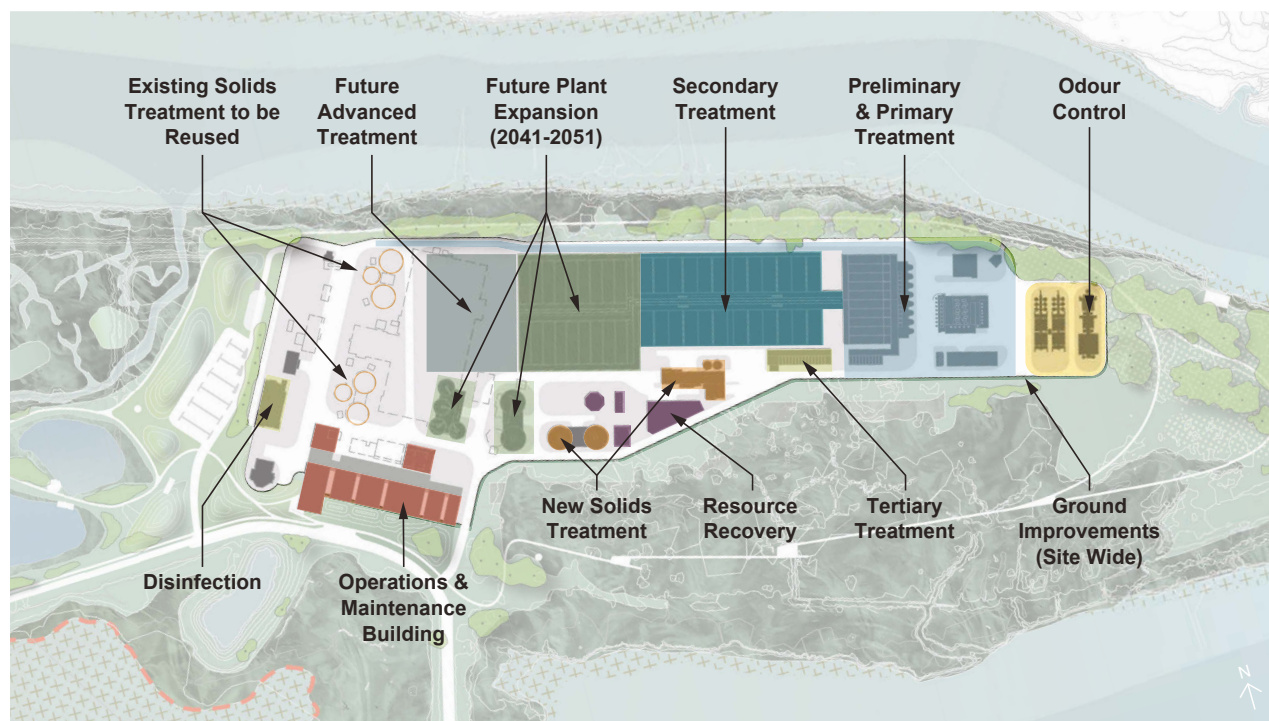
Figure 6. Key components of the proposed IWWTP. **NOTE: Drawings as shown are conceptual and subject to additional study and design development.
