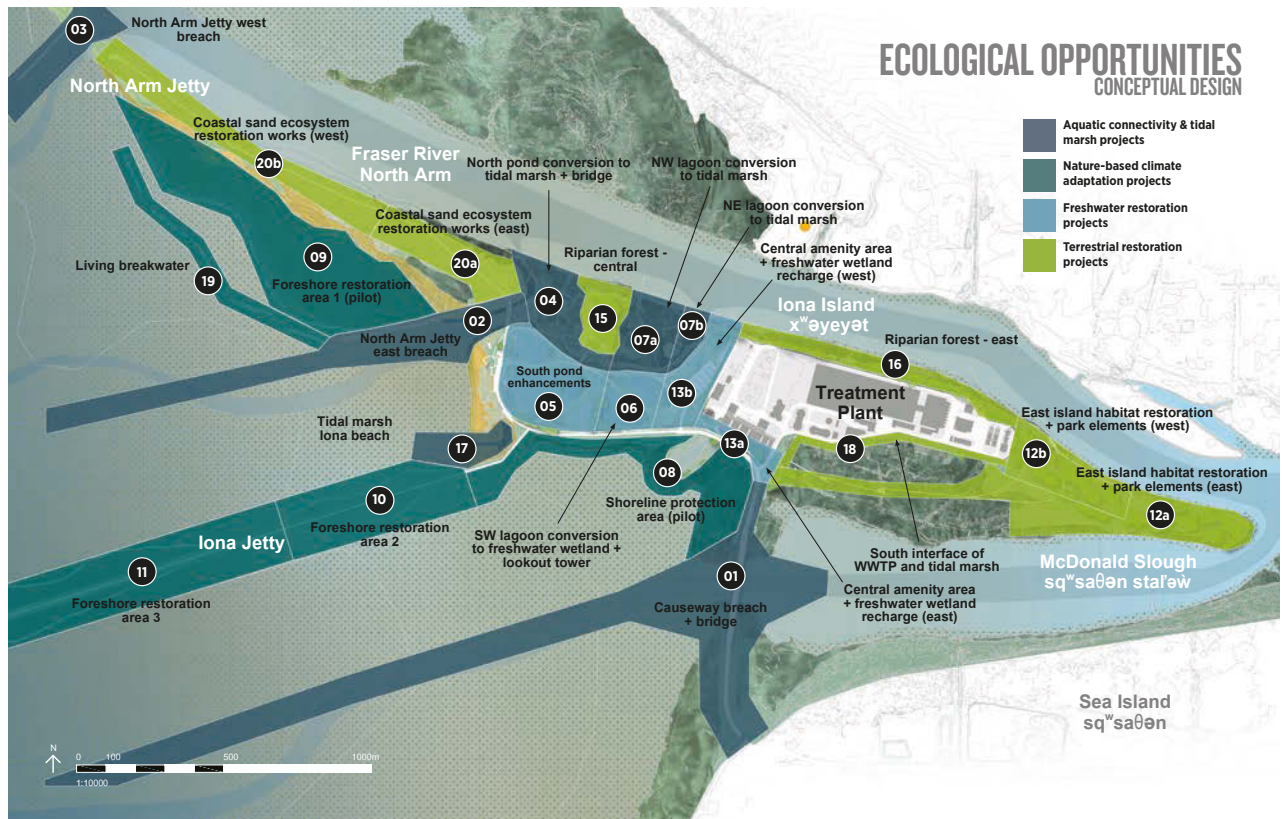
Figure 35. Summary of the ecological restoration projects contemplated as part of the IIWWTP Projects. **NOTE: Drawings as shown are conceptual and subject to additional study and design development.
